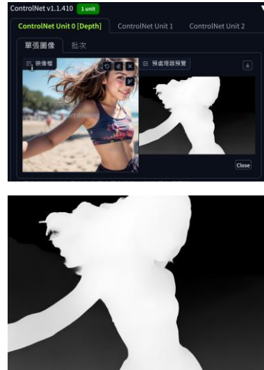
Depth
