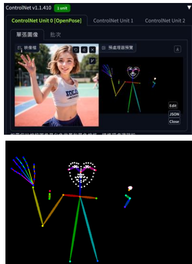
OpenPose
